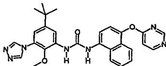
1-(5-tert-Butyl-2-methoxy-3-[1,2,4]triazol-4-yl-phenyl)-3-[4-(pyrimidin-4-yloxy)-naphthalen-1-yl]-urea;
